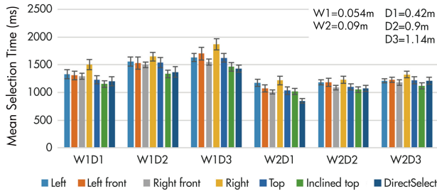
Figure 6: Selection time grouped by TARGETSIZE x TARGETDISTANCE. Each color represents a MIRRORPOSITION.
